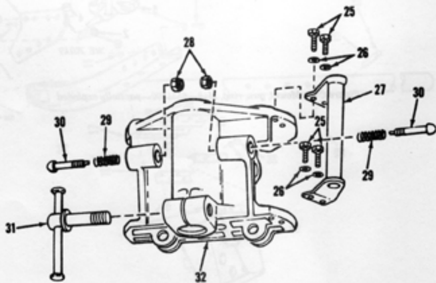
Figure C-17. Carriage assembly—6540721—exploded view.
